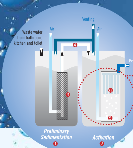
Fig. 3: Diagram of the microfiltration technology
