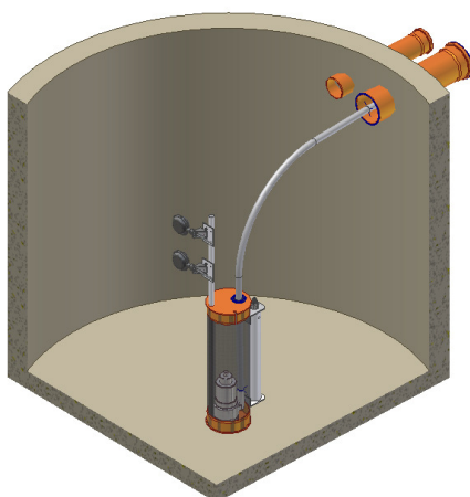
Scheme of the septic tank with coarse matter separator
