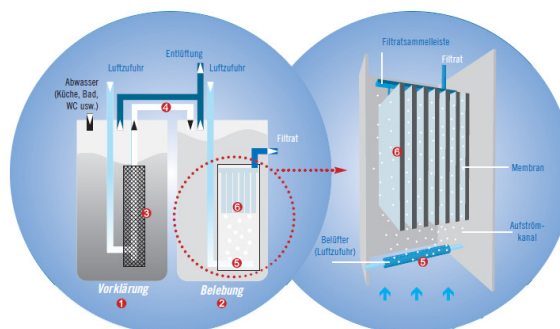
Process design of the BUSSE-MF technology
